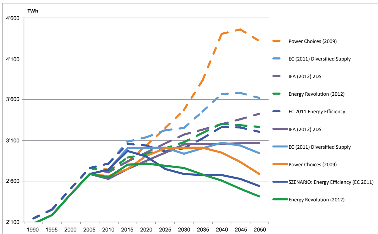
Figure 3. Electricity demand in the decarbonisation scenarios with (dashed lines) and without (bold lines) the transport sector. Sources: Own figure, based on data from respective scenario studies and for historical data from Eurostat (2012).
